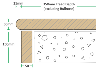
Section of Examples A, B & C
