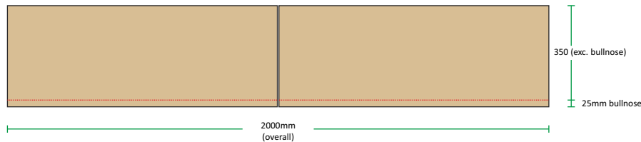
Section of Examples D, E & F
