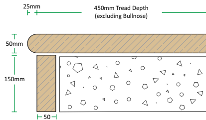
Section of Examples D, E & F
